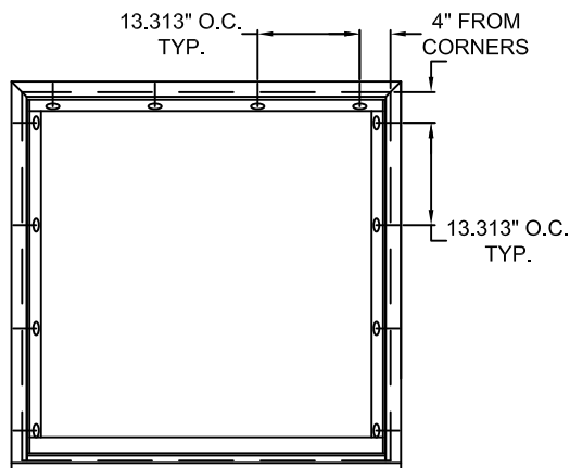
TYPICAL ELEVATION WITH FASTENER SPACING
